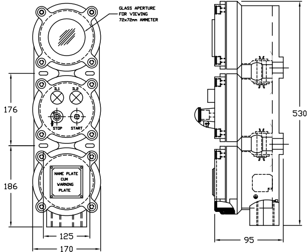
PUSH BUTTON WITH AMMETER
