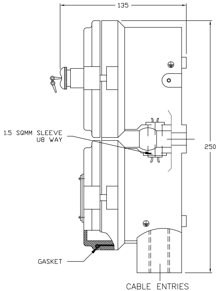
SIDE VIEW
